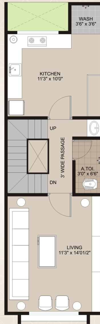
1st FLOOR PLAN
