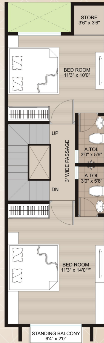
2nd FLOOR PLAN
