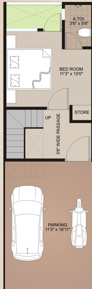
GR. FLOOR PLAN
