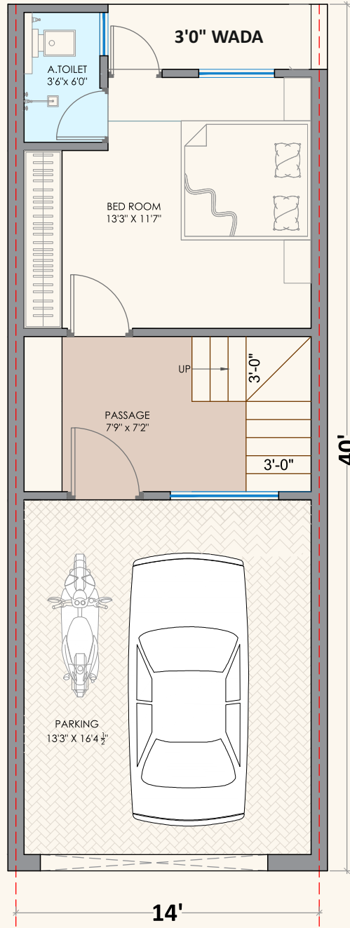
GROUND FLOOR
