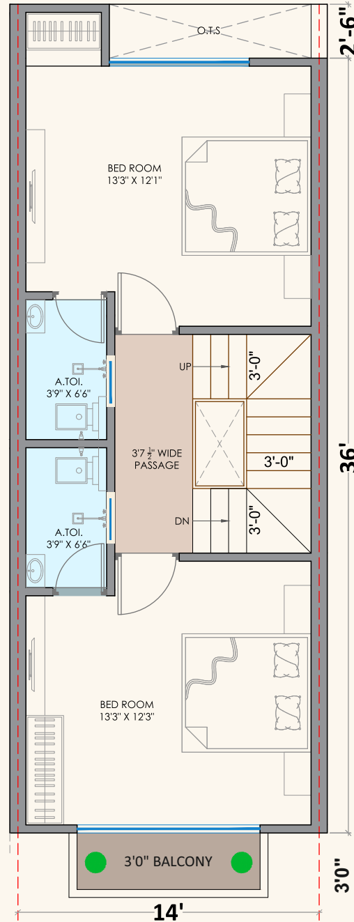
SECOND FLOOR
