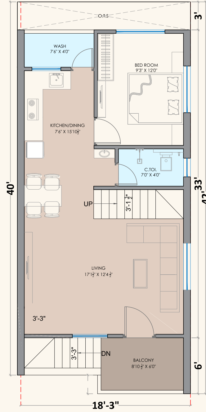
FIRST FLOOR
